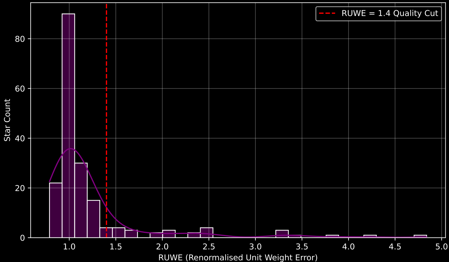
GAPOGEE DR17 Field [032+81_MGA] RUWE Distribution (n= 186)
