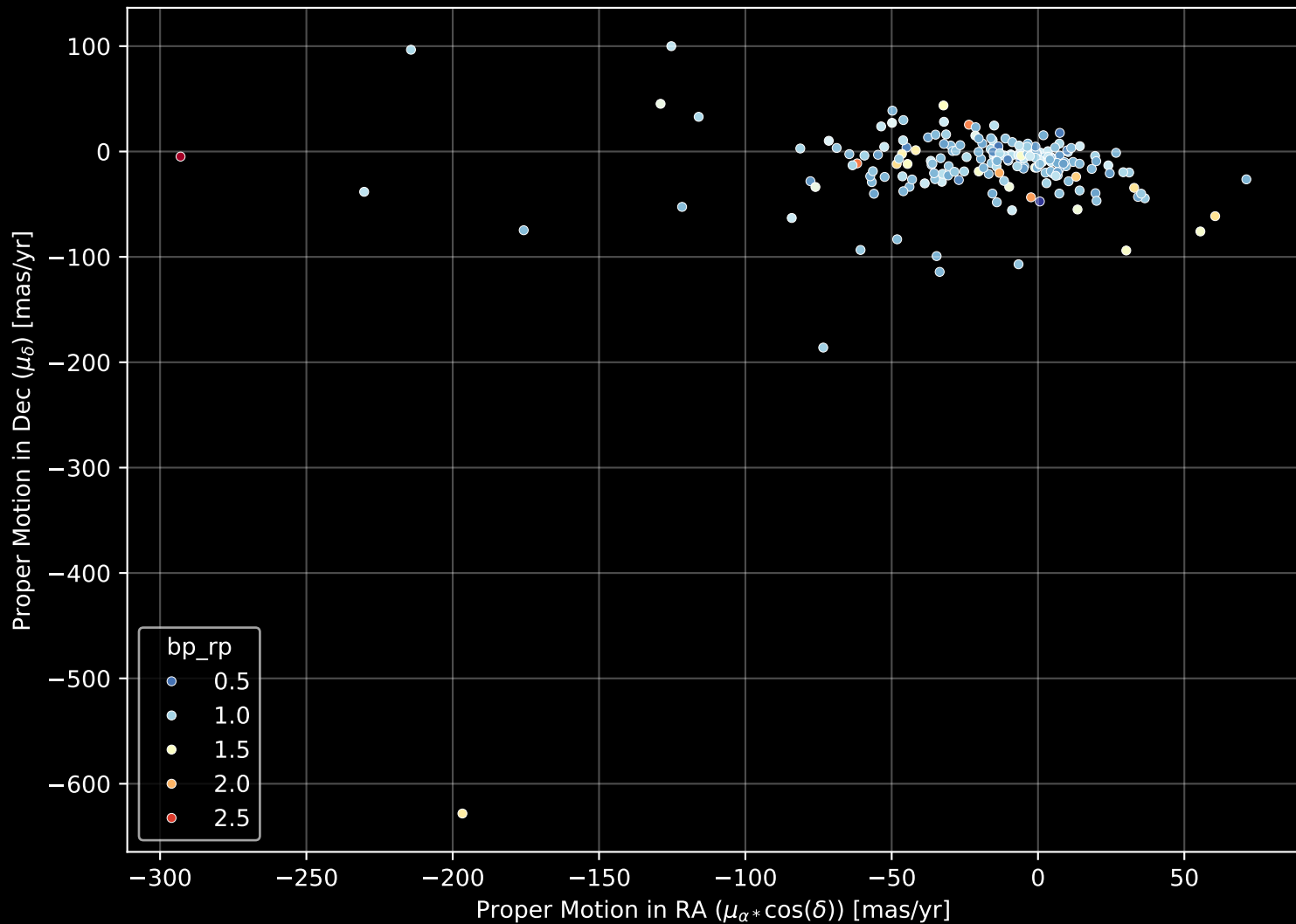
APOGEE DR17 Field: [032+81_MGA] Proper Motion Diagram (n= 198)
