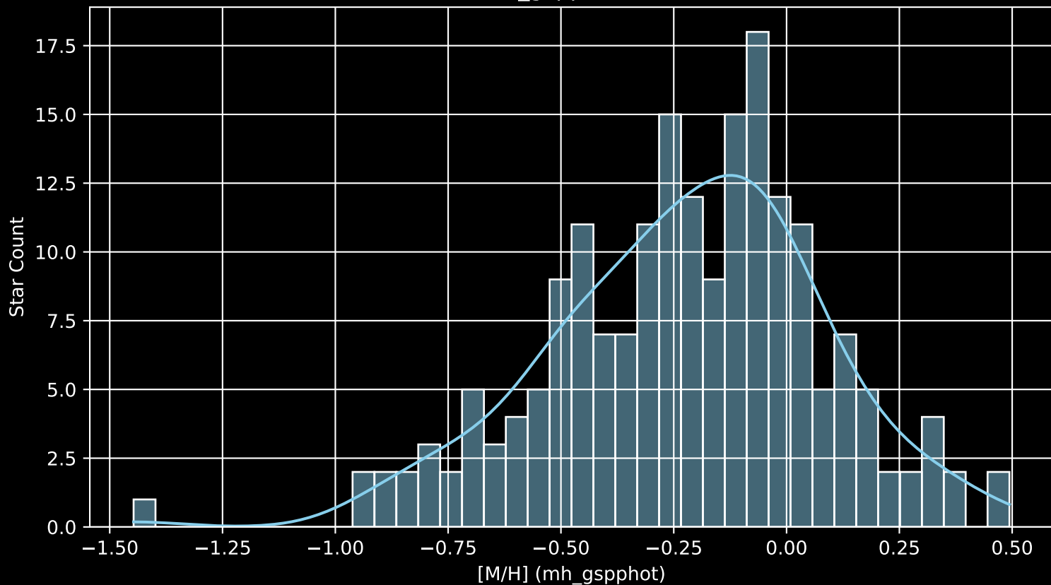
APOGEE DR17 Field: [032+81_MGA [M/H] (mh_gspphot) (n= 195)
