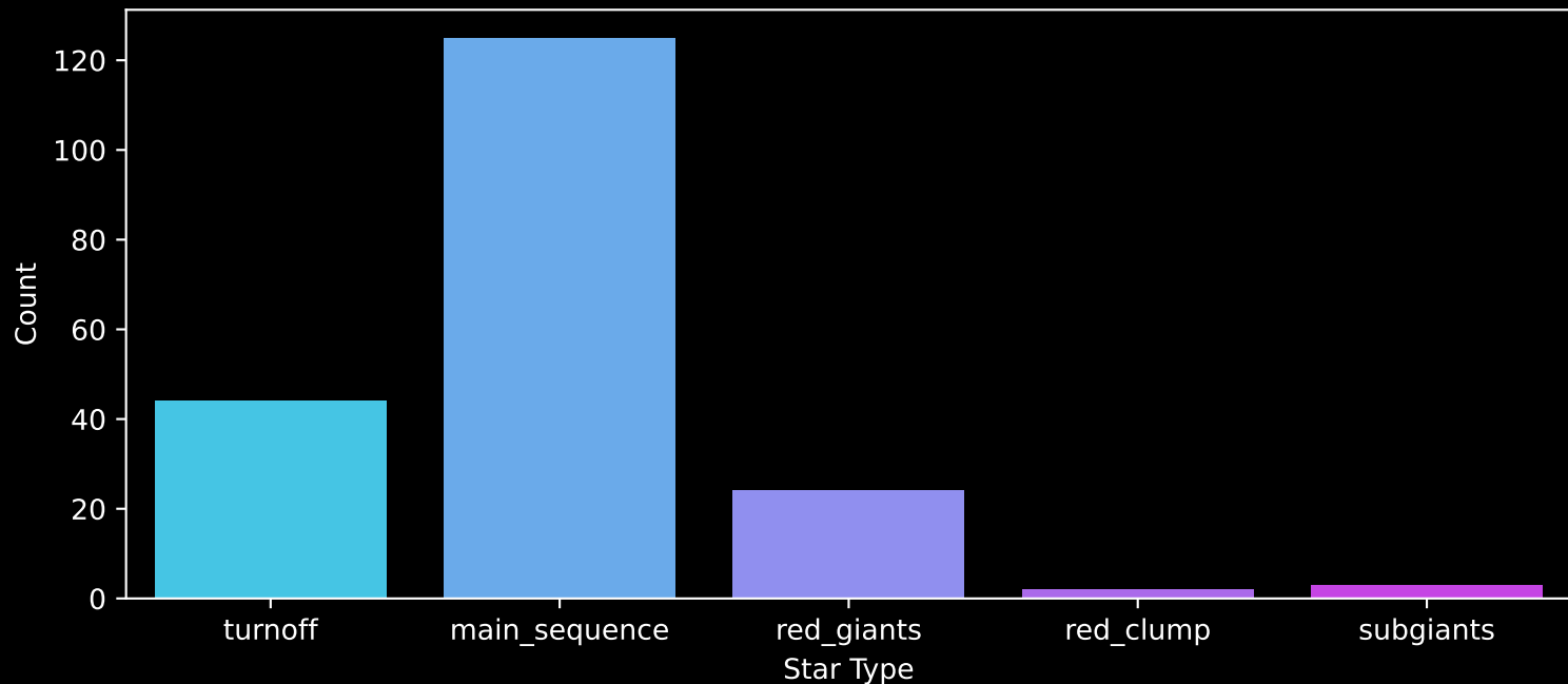
APOGEE DR17 Field: [032+81_MGA] Count plot of Star Type
