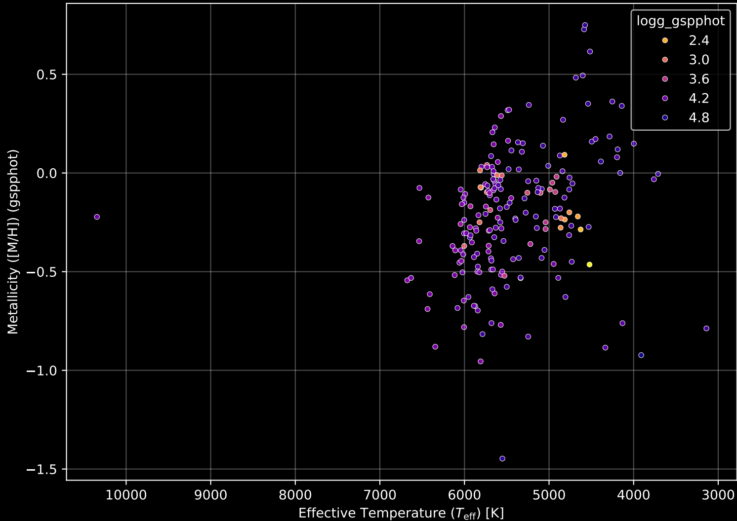
APOGEE DR17 Field: [032+81_MGA] Stellar Population Parameters (n= 198)
