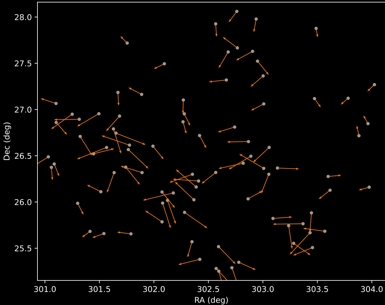
APOGEE DR17 Cluster 2 Proper Motion Vectors (n=87)
