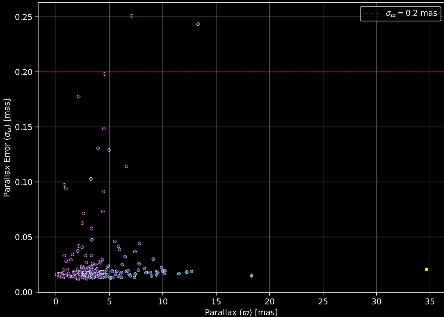
APOGEE DR17 Field: [032+81_MGA] Parallax Quality (n= 198)
